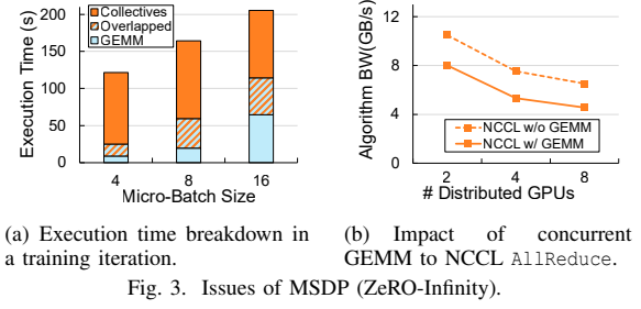
Fig. 3. Issues of MSDP (ZeRO-Infinity).
