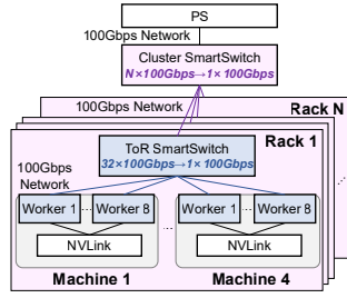
Fig. 12. Multi-rack topology of DisDP.
