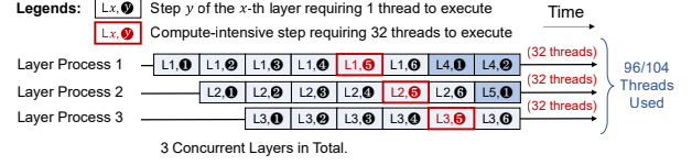
(a) Layer-centric pipelining: Limited parallelism causes pipeline bubbles.
