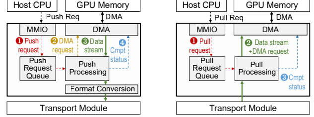
(a) Pushing gradients
