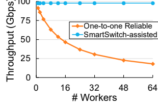
Fig. 8. Throughput under different reliable protocols.
