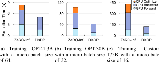
Fig. 17. Execution breakdown comparison.
