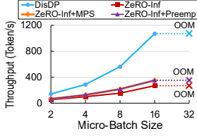
Fig. 21. DisDP vs. simulated ZeRO-Infinity w/o computing unit contention.
