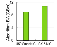
Fig. 20. DMA capability comparison.
