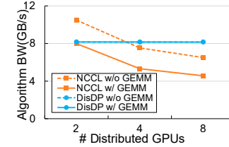
Fig. 19. Algorithm bandwidth of different collective primitives.
