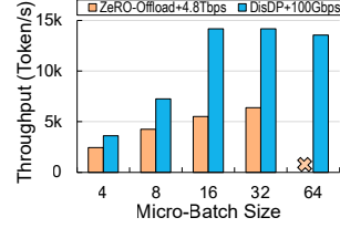
Fig. 27. DisDP 100Gbps network vs. ZeRO-Offload under 4.8Tbps NVLink.
