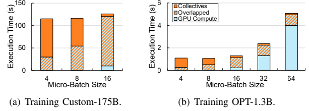
Fig. 18. Breakdown of compute and collectives running DisDP.
