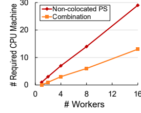
Fig. 5. Overhead of MiSDP: Many extra CPU machines.
