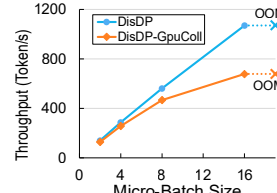
Fig. 23. Effect of interference-free collectives.
